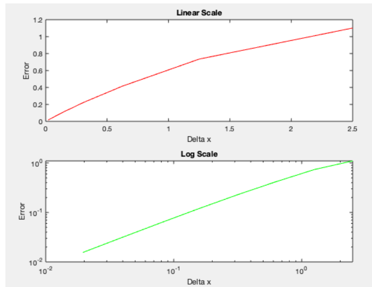
Figure 12: error-analysis
